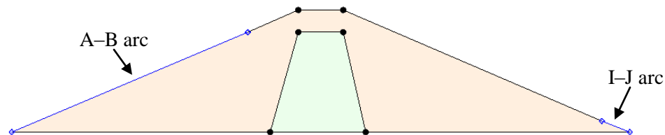
Figure 7 Specified-head boundaries
