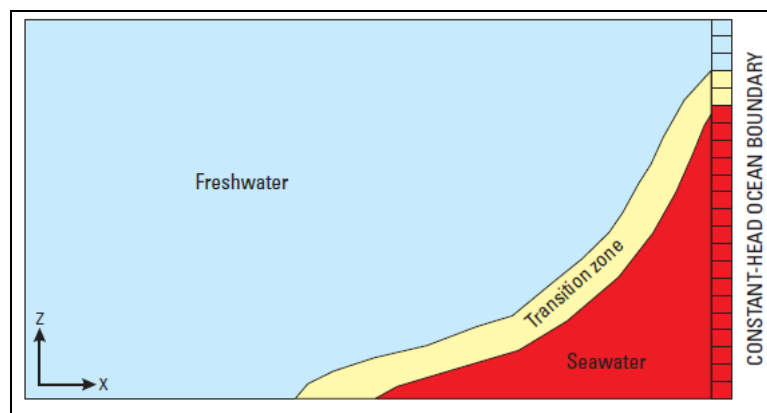
Figure 1 Site to be modeled with SEAWAT
