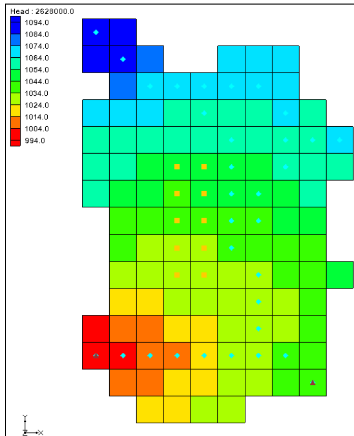
Figure 3 MODFLOW solution
