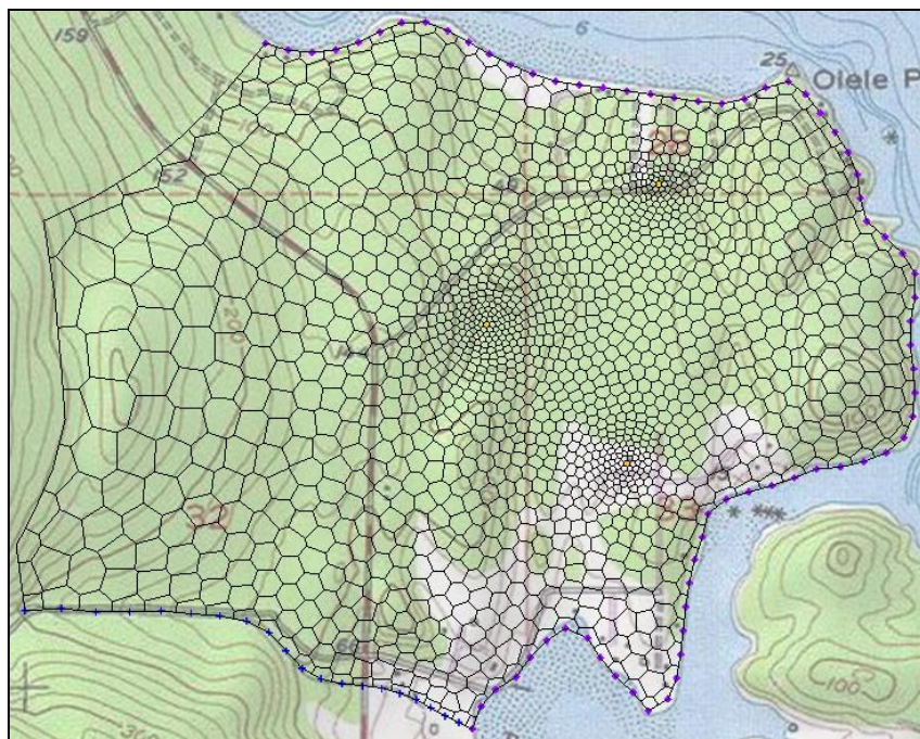
Figure 14 MODFLOW boundary conditions on a Voronoi UGrid
