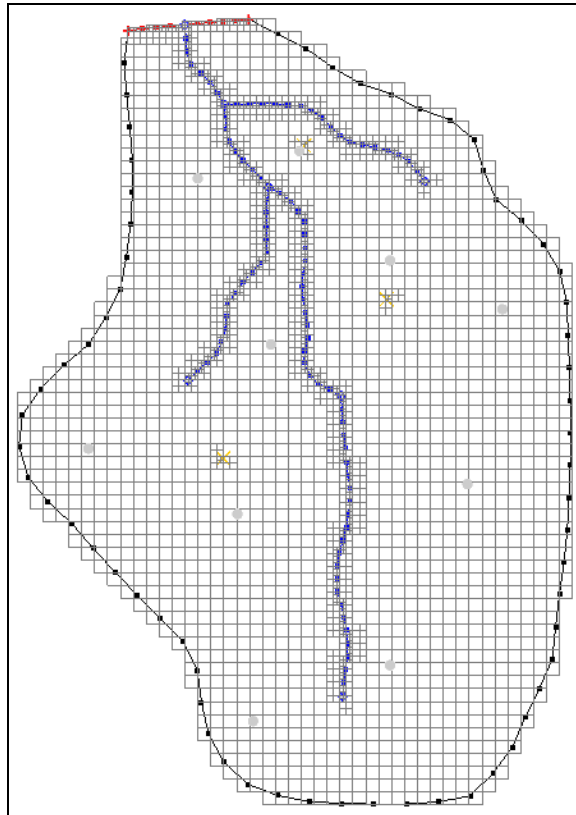
Figure 9 Quadtree UGrid
