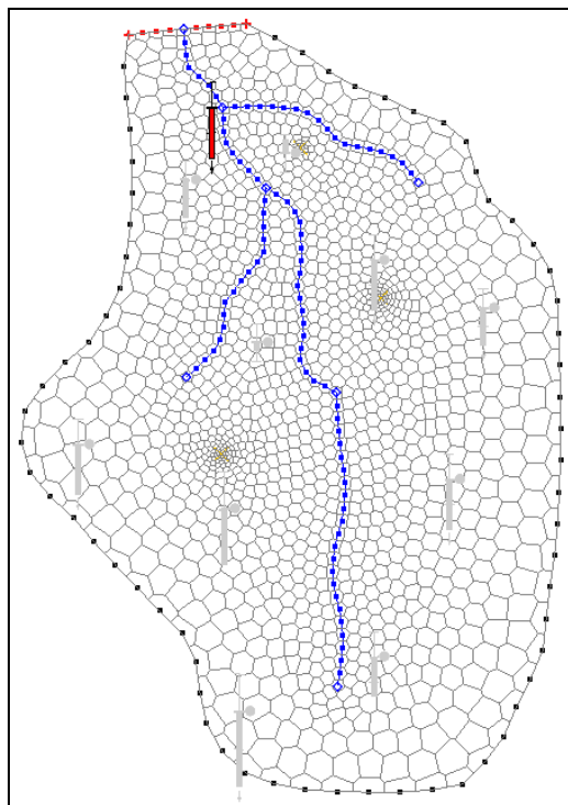
Figure 8 Voronoi UGrid
