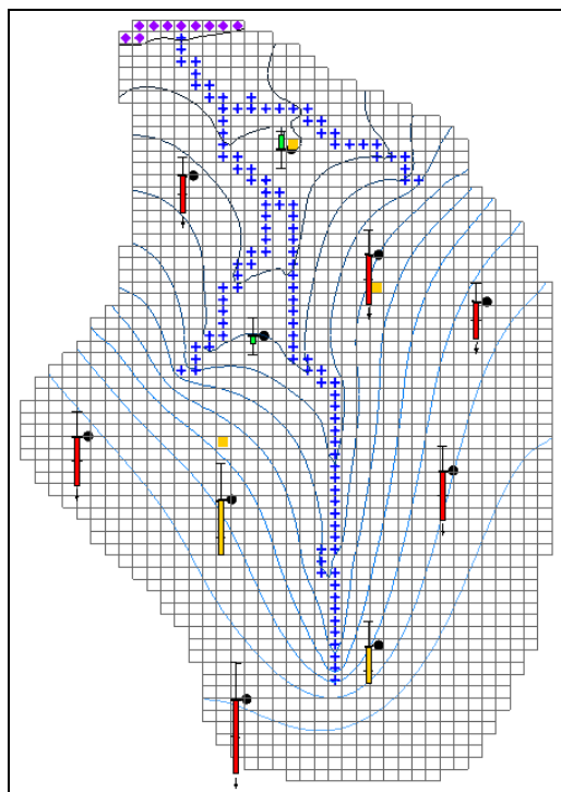
Figure 1 MODFLOW-2000 model
